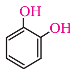
Dihydric
