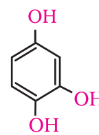
Trihydric
