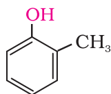
Monohydric
