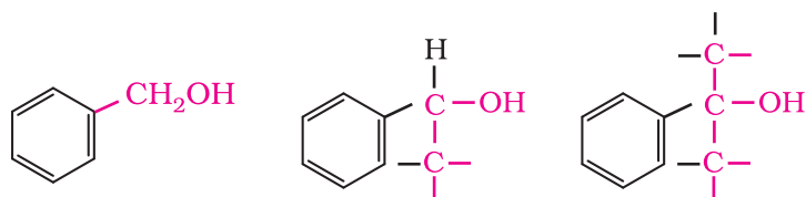
Primary
