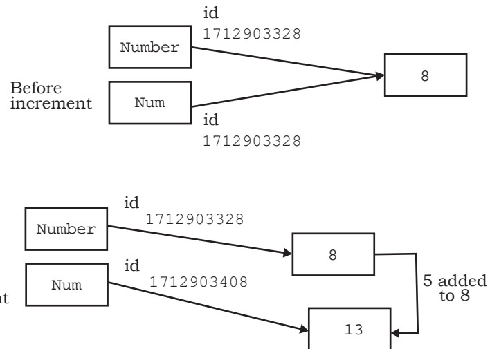
Figure 7.4: ID of argument and parameter before and after increment
